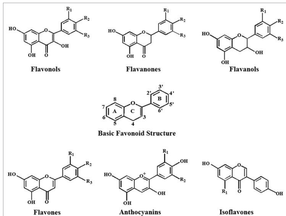
Figure 3. Chemical structures of sub-classes of flavonoids. Based on the variation in the type of heterocycle involved, flavonoids are divided into six major subclasses: flavonols, flavanones, flavanols, flavones, anthocyanins and isoflavones. Individual differences within each group arise from the variation in number and arrangement of the hydroxyl groups and their extent of alkylation and/or glycosylation. Flavonols (such as quercetin and kaempferol), have a 3-hydroxy pyran-4-one group on the C ring. Flavanones (such as naringenin and taxifolin), have an unsaturated carbon-carbon bond in the C ring. Flavanols (such as the catechins), lack both a 3-hydroxyl group and the 4-one structure in the C ring. Flavones (such as luteolin), lack a hydroxyl group in the 3-position on the C ring. Anthocyanins (such as cyanidin), are characterized by the presence of an oxonium ion on the C ring and are highly coloured as a consequence and in isoflavones (such as genistein), the B ring is attached to the C ring in the 3-position, rather than the 2-position as is the case with the other flavonoids.
