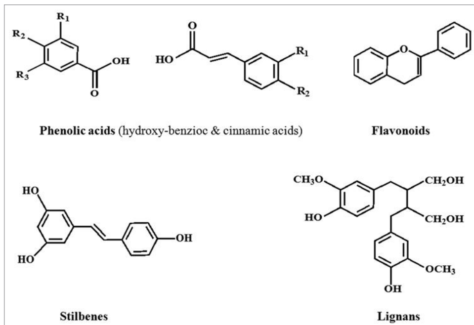
Figure 2. Chemical structures of the different classes of polyphenols. Polyphenols are classified on the basis of the number of phenol rings that they contain and of the structural elements that bind these rings to one another. They are broadly divided in four classes; Phenolic acids, flavonoids, stilbenes and lignans. Phenolic acids are further divided into hydroxyl benzoic and hydroxyl cinnamic acids. Phenolic acids account for about a third of the polyphenolic compounds in our diet and are found in all plant material, but are particularly abundant in acidic-tasting fruits. Caffeic acid, gallic acid, ferulic acid are some common phenolic acids. Flavonoids are most abundant polyphenols in human diet and share a common basic structure consist of two aromatic rings, which are bound together by three carbon atoms that form an oxygenated heterocycle. Biogenetically, one ring usually arises from a molecule of resorcinol, and other ring is derived from the shikimate pathway. Stilbenes contain two phenyl moieties connected by a two-carbon methylene bridge. Most stilbenes in plants act as antifungal phytoalexins, compounds that are synthesized only in response to infection or injury. The most extensively studied stilbene is resveratrol. Lignans are diphenolic compounds that contain a 2,3-dibenzylbutane structure that is formed by the dimerization of two cinnamic acid residues.
